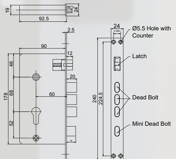
60 x 68mm Lock Body
